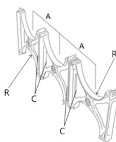
INTERMEDIATE SPACER
