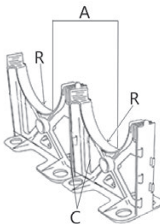
BASE SPACER
